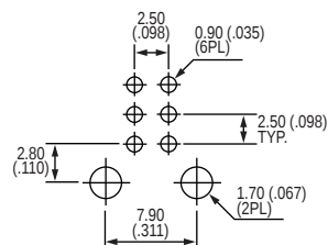
PC Layout
